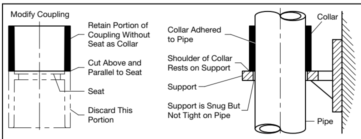
Figure 6 - Riser Collar
