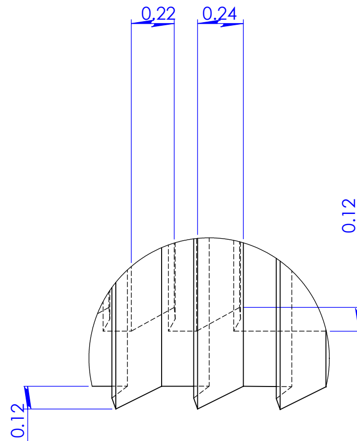
DETAIL A SCALE 2 : 1
