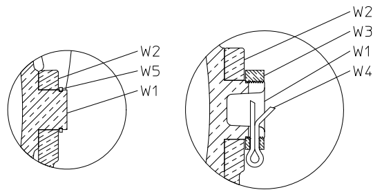
3" THRU 6" SIZES
