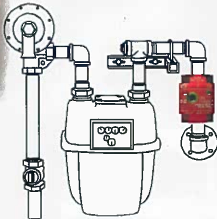
VAGV Series Vertical Gas Safety Valve
