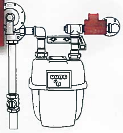
AGV Series Horizontal Gas Safety Valve
