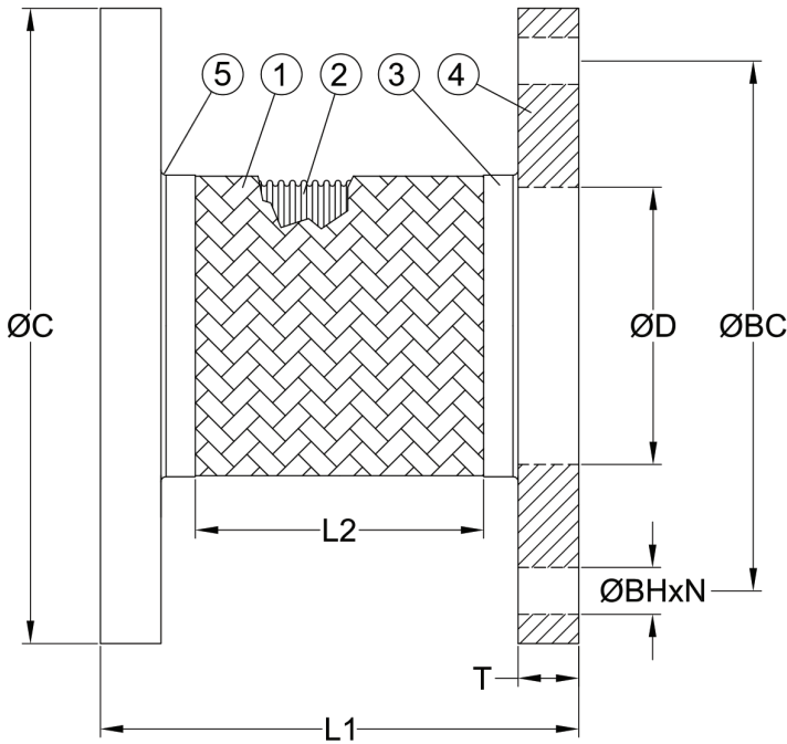
PARTS NUMBERS & WEIGHT (INCHES)
