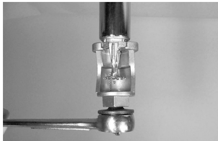
CORRECT ENGAGEMENT FOR MODEL V36 RECESSED WRENCH
