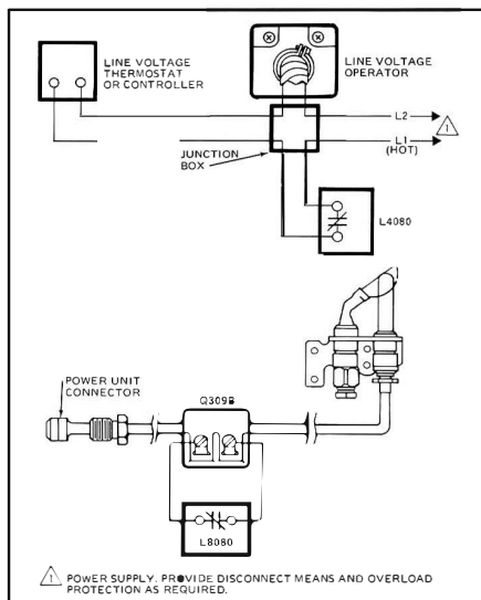
Fig. 4. Typical wiring hookup for line voltage system.
