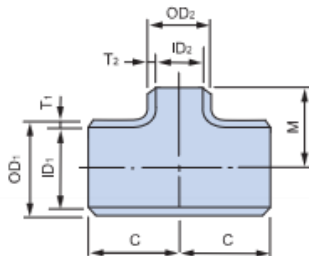
(REDUCING)
