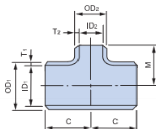
(REDUCING)
