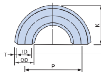
180°ELBOW
