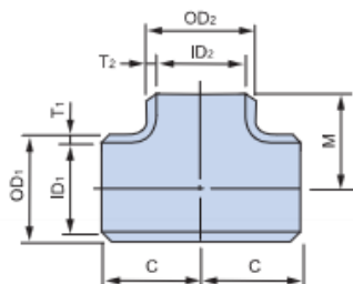
(STRAIGHT)
