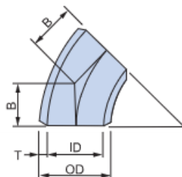
45°ELBOW
