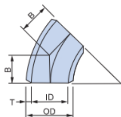
45°ELBOW
