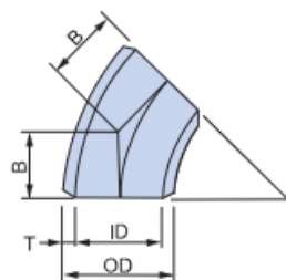
45°ELBOW
