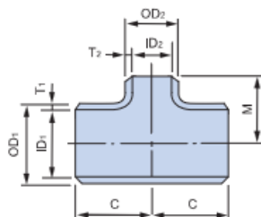
(REDUCING)
