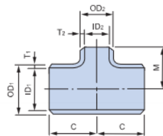
(REDUCING)
