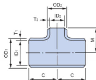
(REDUCING)
