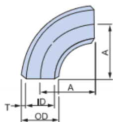
90°ELBOW (LONG)
