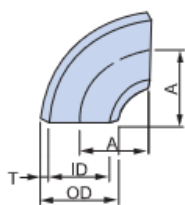
90°ELBOW (SHORT)
