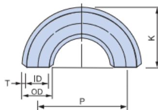
180°ELBOW
