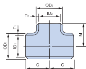
(STRAIGHT)
