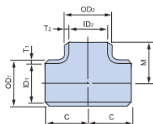
(STRAIGHT)
