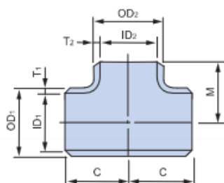
(STRAIGHT)
