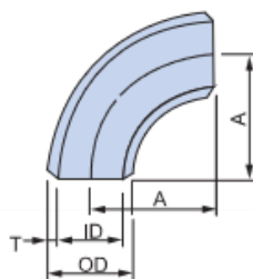
90°ELBOW (LONG)
