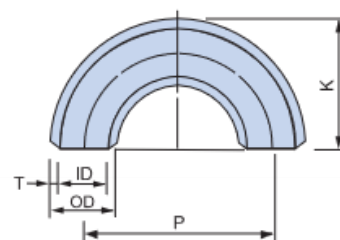
180°ELBOW
