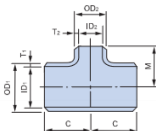
(REDUCING)
