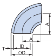
90°ELBOW (SHORT)
