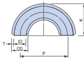
180°ELBOW
