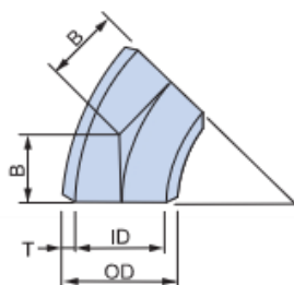
45°ELBOW
