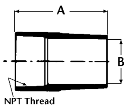
Adapter - Spigot x Female
