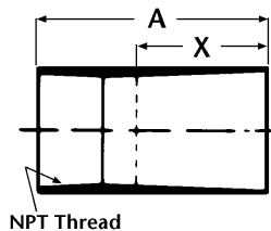
Adapter (Male x Female)
