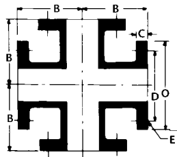
Cross - Flanged
