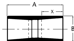
Sleeve Coupling
