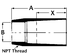
Adapter (Bell x Male)
