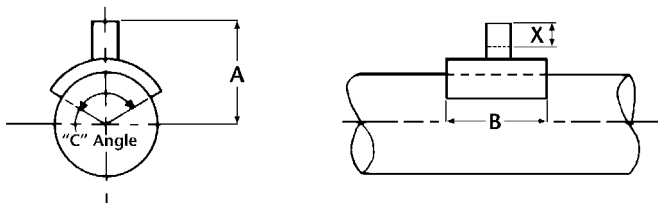
Saddle - Belled Side Outlet
