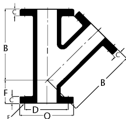
45° Lateral Flanged
