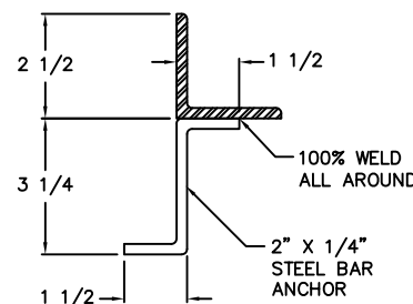
ANCHOR DETAIL
