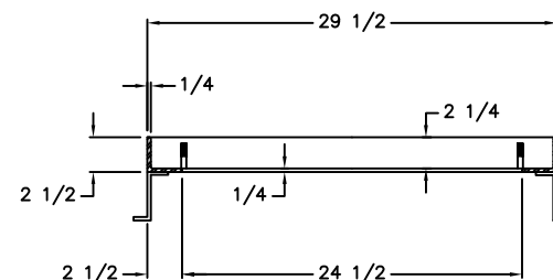
FRAME SECTION
