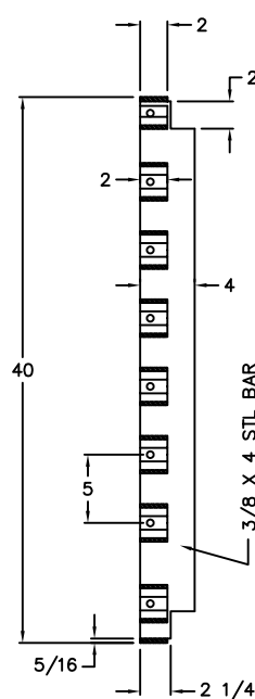
GRATE SECTION
