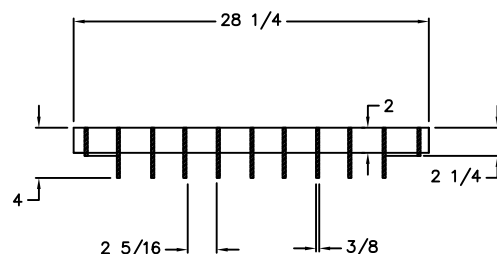
GRATE SECTION
