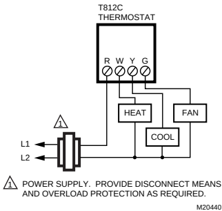
Fig. 7. T812C in heating and cooling system.
