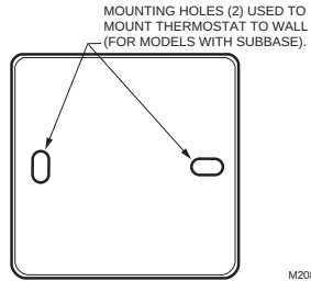
Fig. 3. Mounting hole locations for models with subbase.
