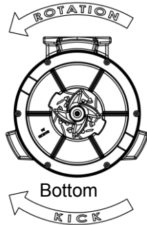
Fig. A – Proper impeller rotation, three phase models
