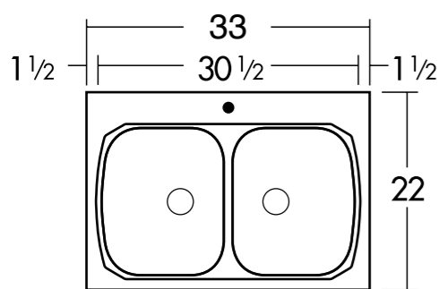
Maxi Basin 1 13 3/4 x 16 1/2 x 8" deep 6.2 Gallon Capacity
