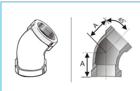
45 Elbow
