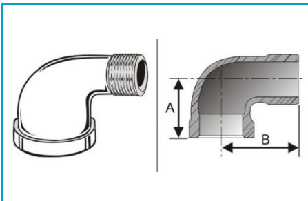
90 Street Elbow
