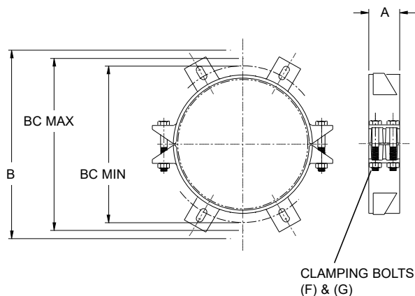
1300 SPLIT RESTRAINT
