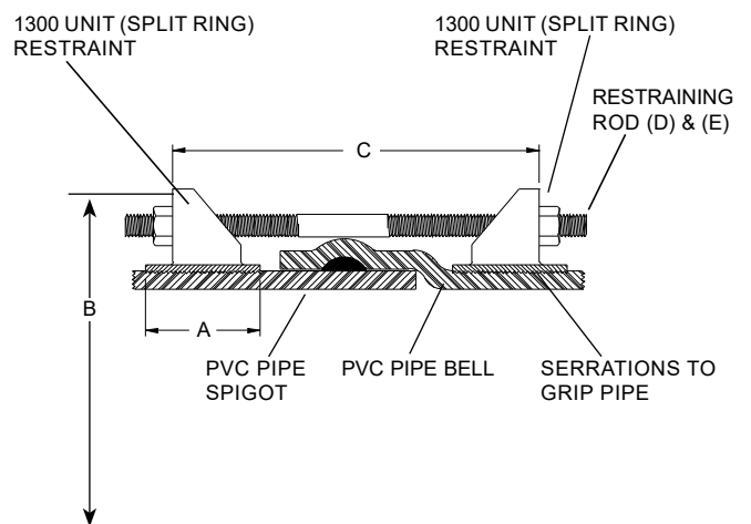
1390 ASSEMBLY
