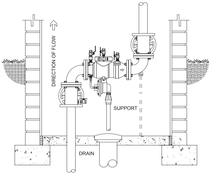
INDOOR INSTALLATION
