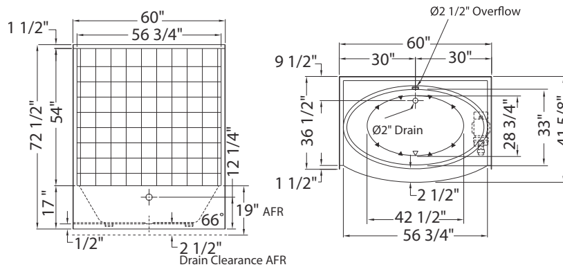
GTWT-4260 Center drain model
