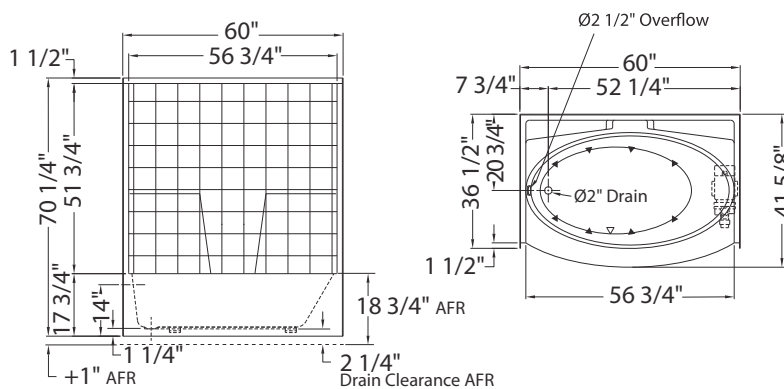
GTWT-4260 Left and right hand drain model
