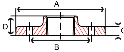
Fig. 17RT1 & 18RT1 – 125 lb. Reducing Companion Flange
