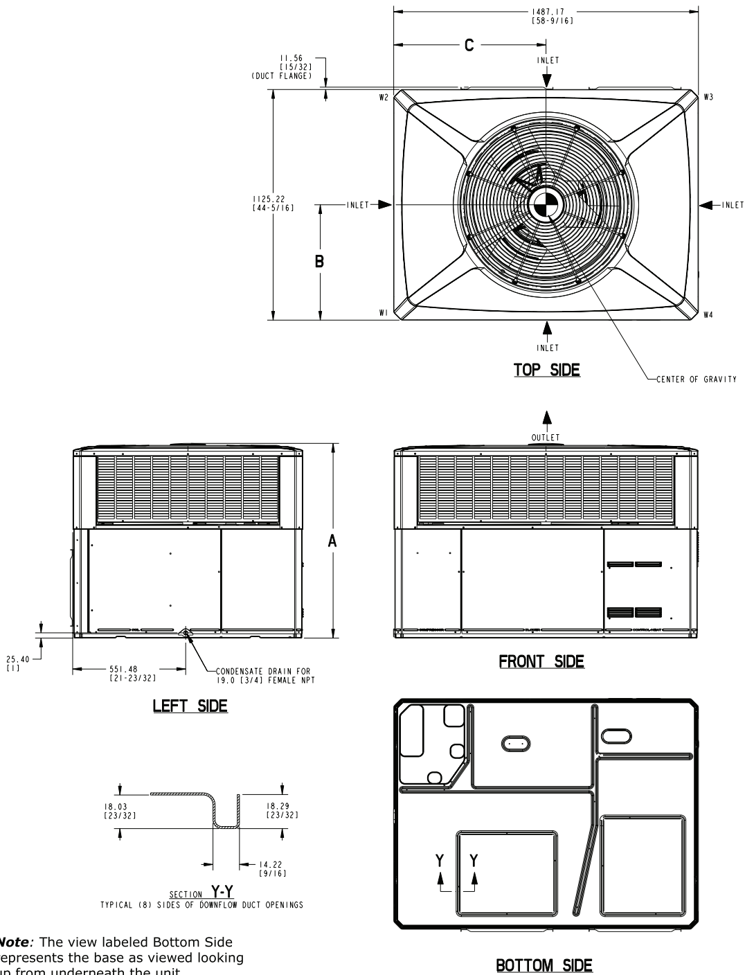
Figure 12. 3.5 – 5 TON MODELS
