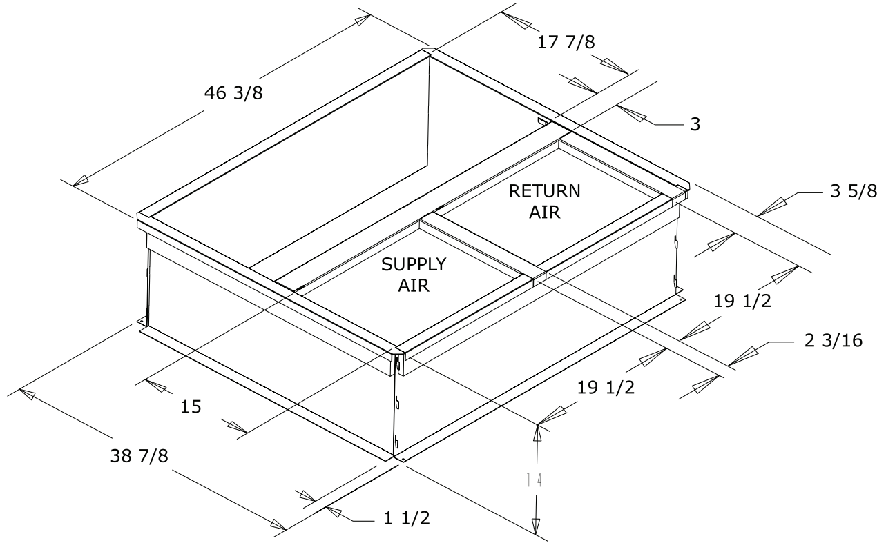
Figure 5. 4024 – 4036 Models
