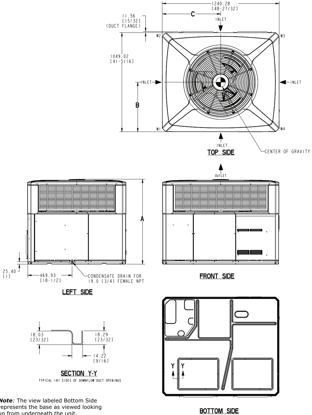
Figure 9. 2 — 3 TON MODELS
