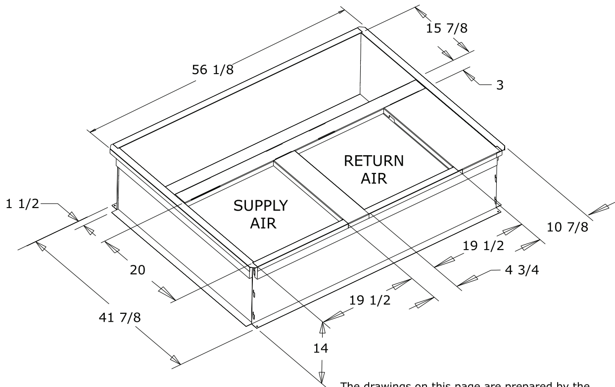
Figure 6. 4042 – 4060 Models
