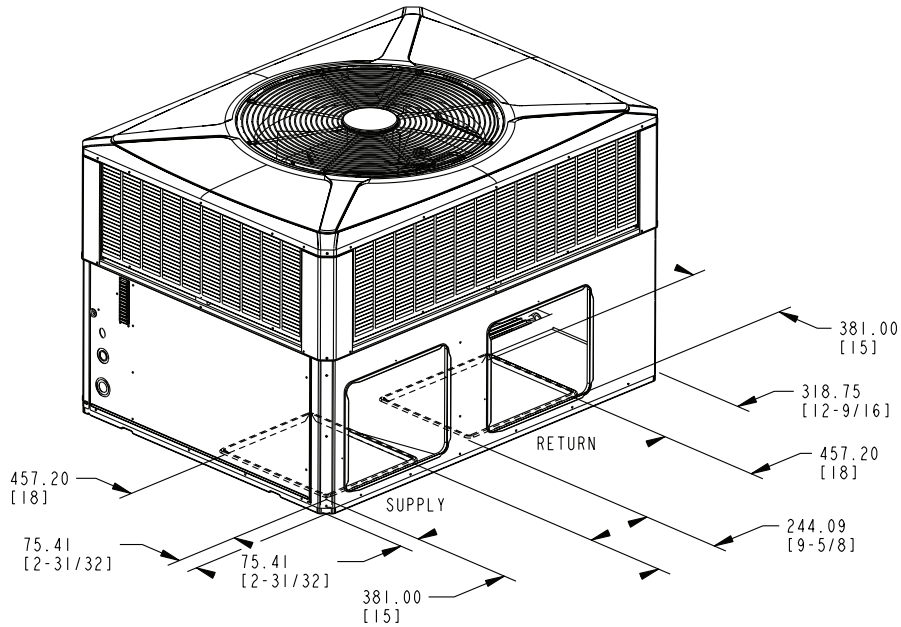
Figure 14. 3.5 – 5 TON MODELS
