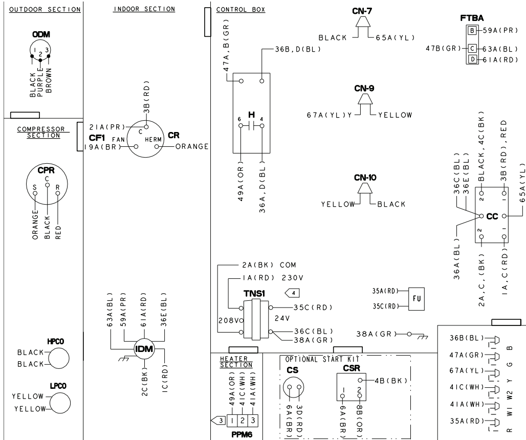
Figure 1. 4TCC4024 — 4042 Models
