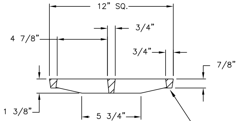
GRATE SECTION
