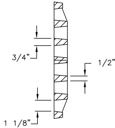
GRATE SECTION
