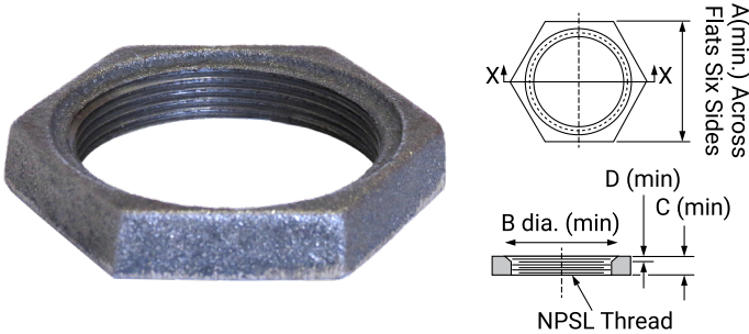
Fig. 1134 Hex Locknut (Class 150 Standard)
