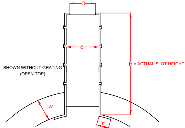
4" - 36" PIPE WITH VARIABLE SLOT RISER DIMENSIONS
