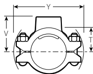
Style 622 Copper Mechanical-T Bolted Branch Outlet
