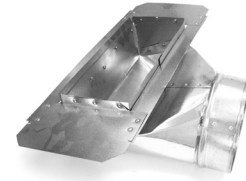
Angle Register Boot with 17" Plate Series 710RP
