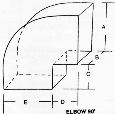
FIG. 5 ELBOW 90° RADIUS HEEL SQUARE THROAT
