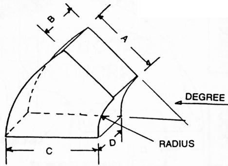
FIG. 9 CHANGE ELBOW RADIUS HEEL & THROAT
