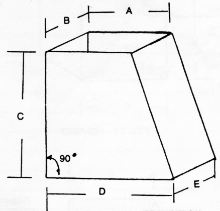
FIG. 6 TRANSITION ONE SIDE STRAIGHT
