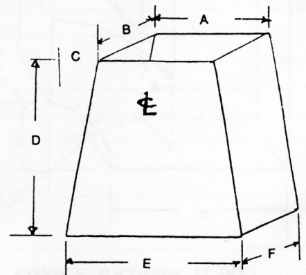
FIG. 8 CENTERLINE TRANSITION TWO SIDES SLOPED
