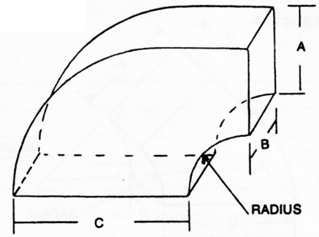
FIG. 2 CHANGE ELBOW 90° RADIUS HEEL & THROAT
