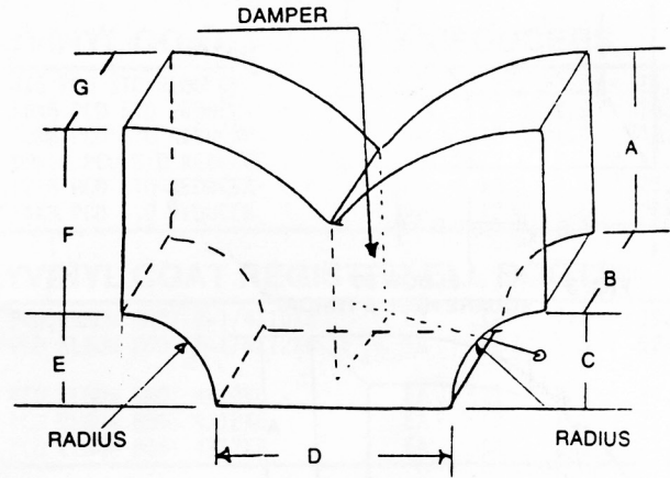
FIG. 12 Y-BRANCH WITH DAMPER RADIUS HEEL & THROAT
