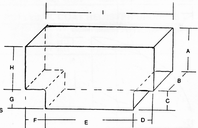
FIG. 14 TEE WITH STRAIGHT HEEL AND SQUARE THROAT
