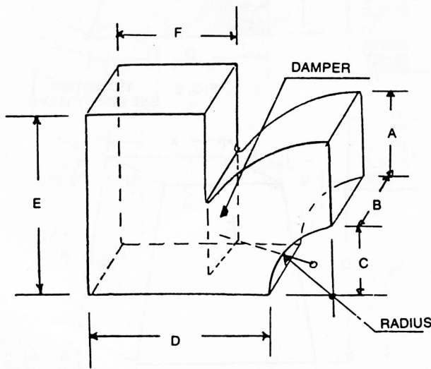
FIG. 13 Y-BRANCH WITH DAMPER AND ONE SIDE STRAIGHT
