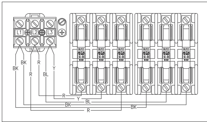
Figure 3. Example of finished Three Phase construction.
