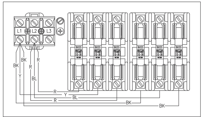
Figure 4. Example of finished Single Phase construction.
