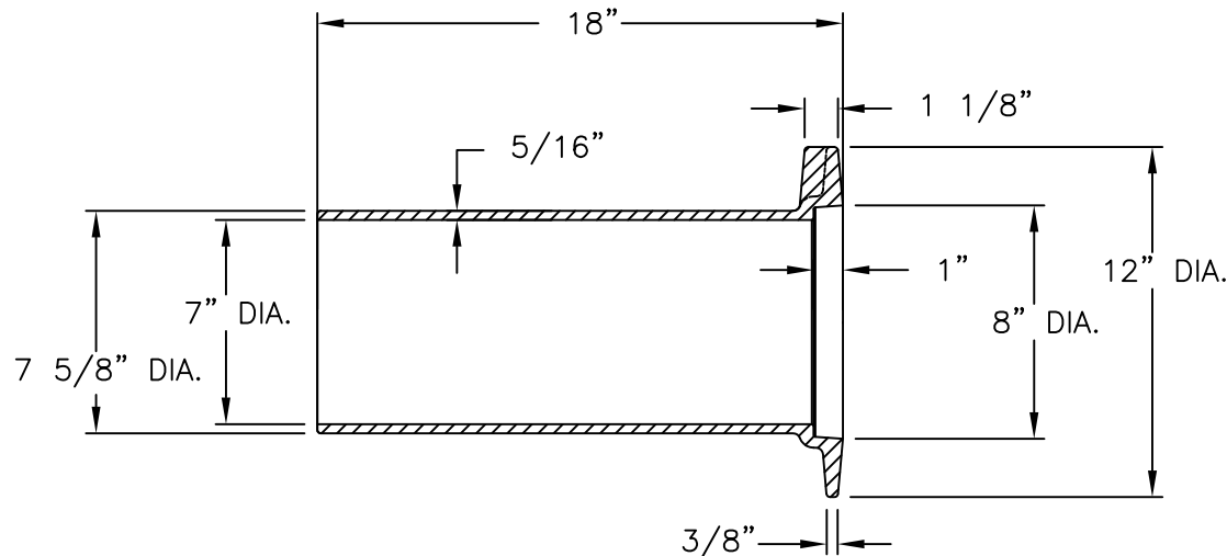
SECTION VIEW
