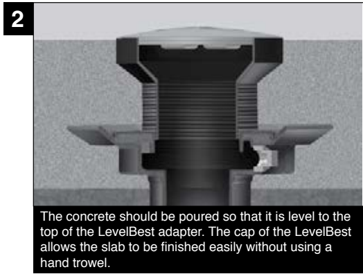
Set drain with LevelBest rough-in adapter at concrete pour level. The height can be adjusted by tightening or loosening the adapter.
