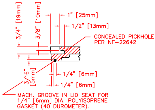
SELF-SEAL DETAIL QUARTER SCALE
