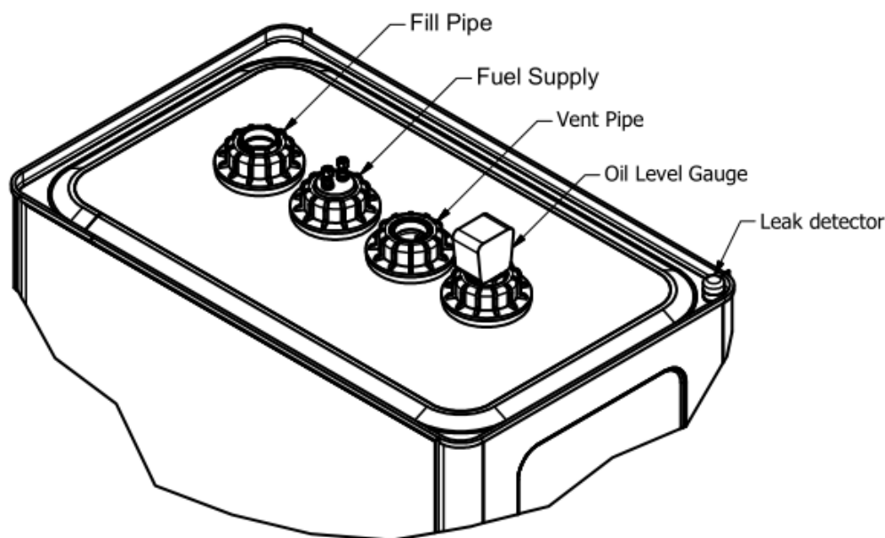
Suggested connection diagram
