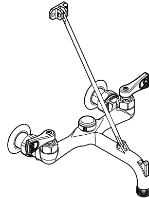
Two-Handle Service Sink Faucet
