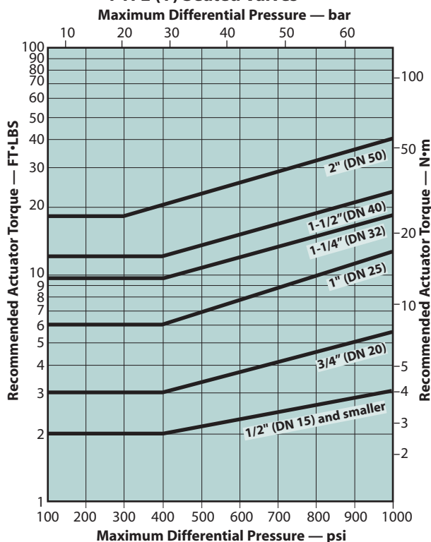
PTFE (T) Seated Valves
