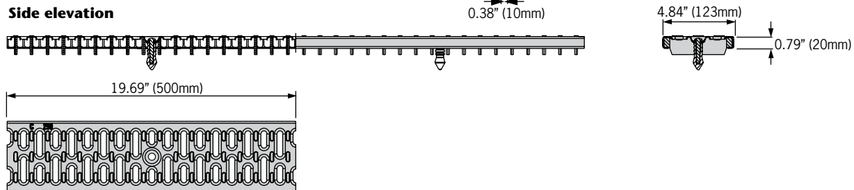
Side elevation
