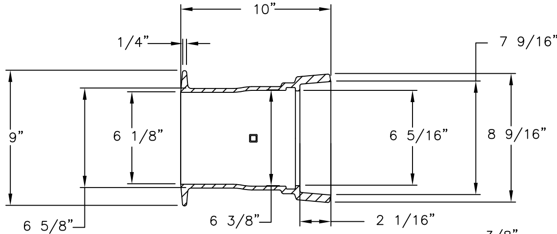
TOP SECTION
