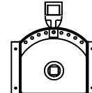
Commercial Damper Extension: 2" H with 9 position locking dial, 18GA construction and 3/8" Rodded Damper
