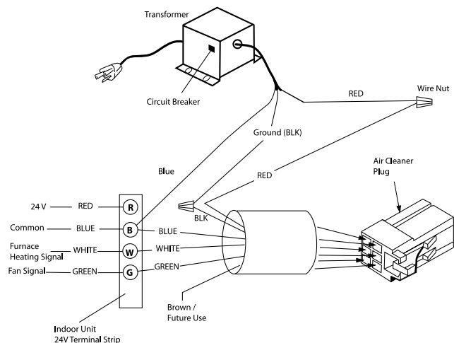
Figure 23 BAYTRANS12024♦ Transformer
