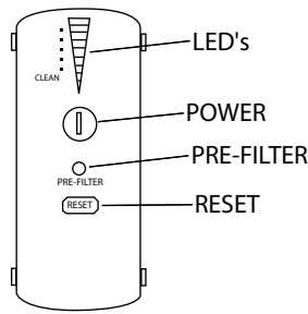
Figure 24 LED Display
