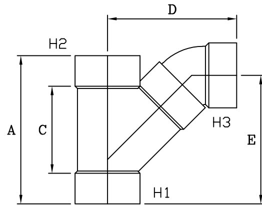
FABRICATED FITTING
