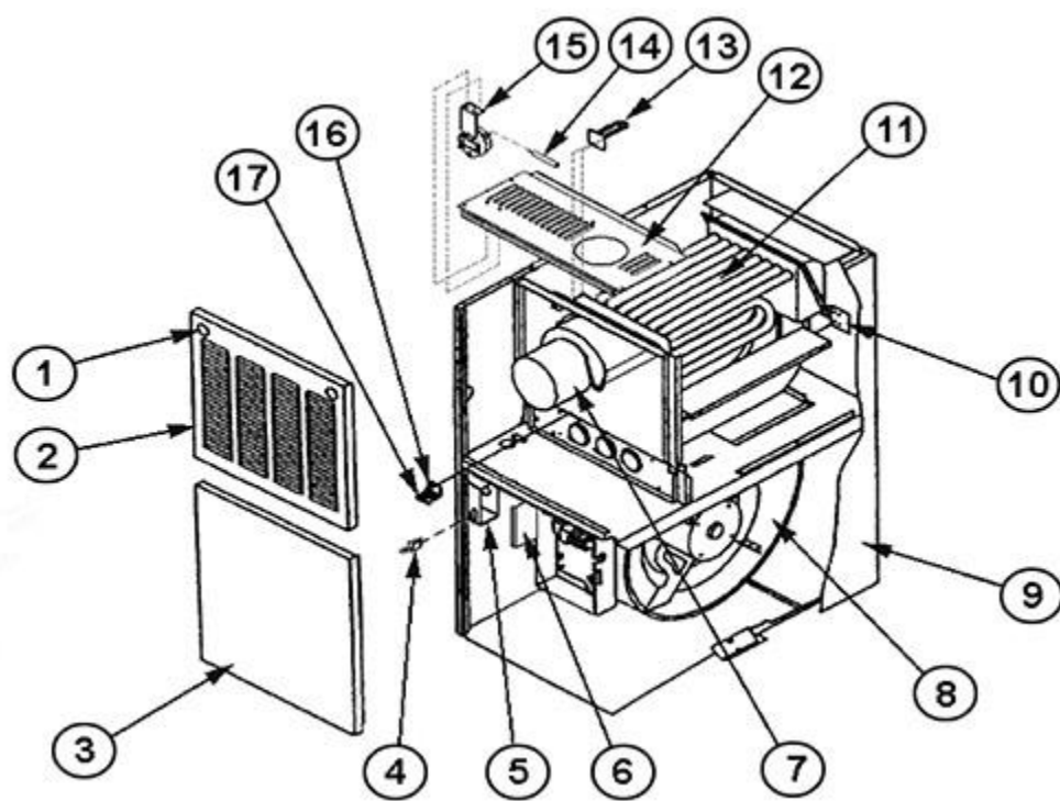
Exploded View
