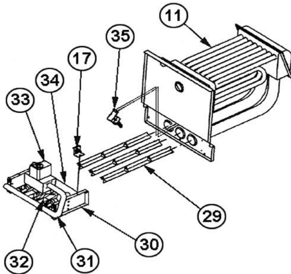
Burner Assembly
