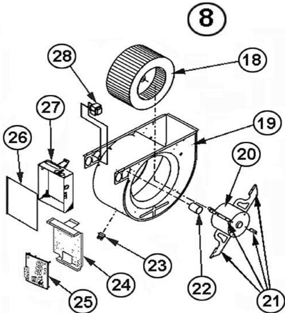
Blower Assembly
