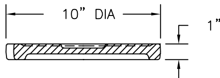
COVER SECTION
