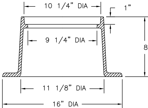
FRAME SECTION
