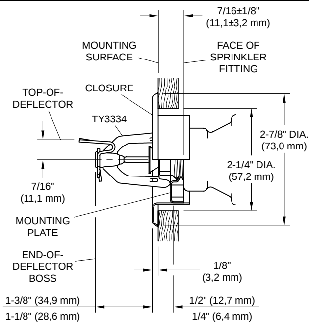
FIGURE 2 STYLE 20 RECESSED ESCUTCHEON FOR USE WITH THE SERIES LFII (TY3334) RESIDENTIAL HORIZONTAL SIDEWALL SPRINKLER
