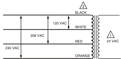
Fig. 11. AT20/AT40 Transformer schematic.
