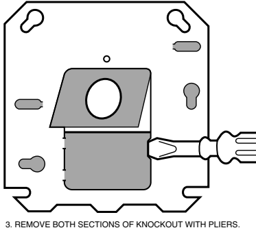
Fig. 6. Removing large center knockout.
