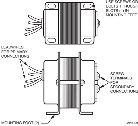
Fig. 10. Foot mounting of AT87 Transformer.
