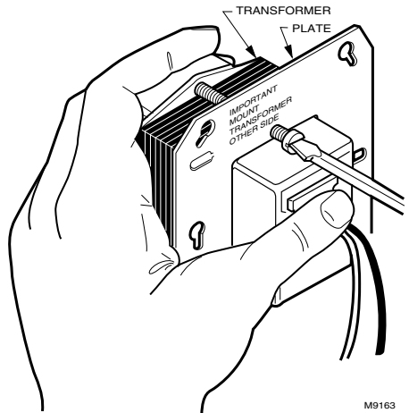
Fig. 8. Secure plate to transformer with mounting screw.
