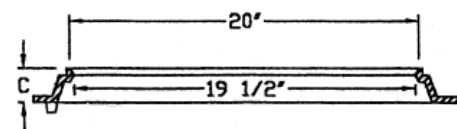
SECTION-XX'
