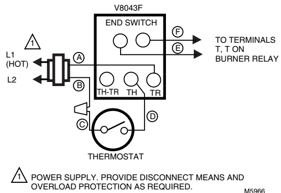
Fig. 31. Wiring Honeywell V8043F to Flair System (two options). (Wires are identified with letters to correspond with wires in Fig. 29.)
