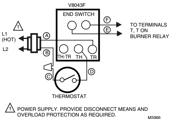
Fig. 28. Wiring Honeywell V8043F to Dole System (two options). (Wires are identified with letters to correspond with wires in Fig. 26.)
