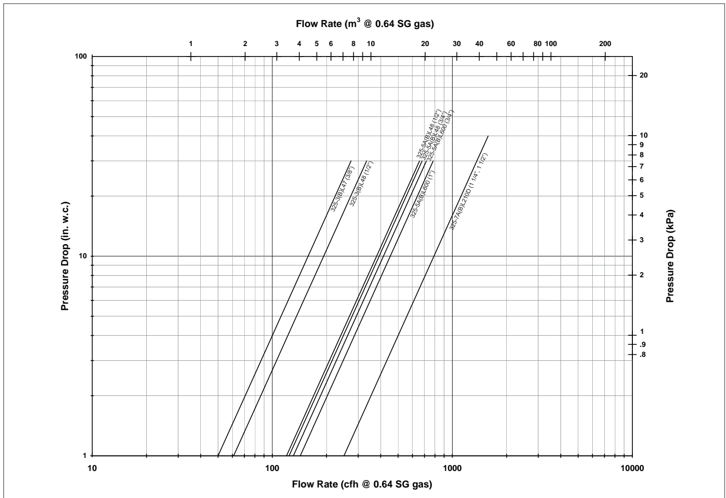
Figure 4: Pressure Drop Chart
