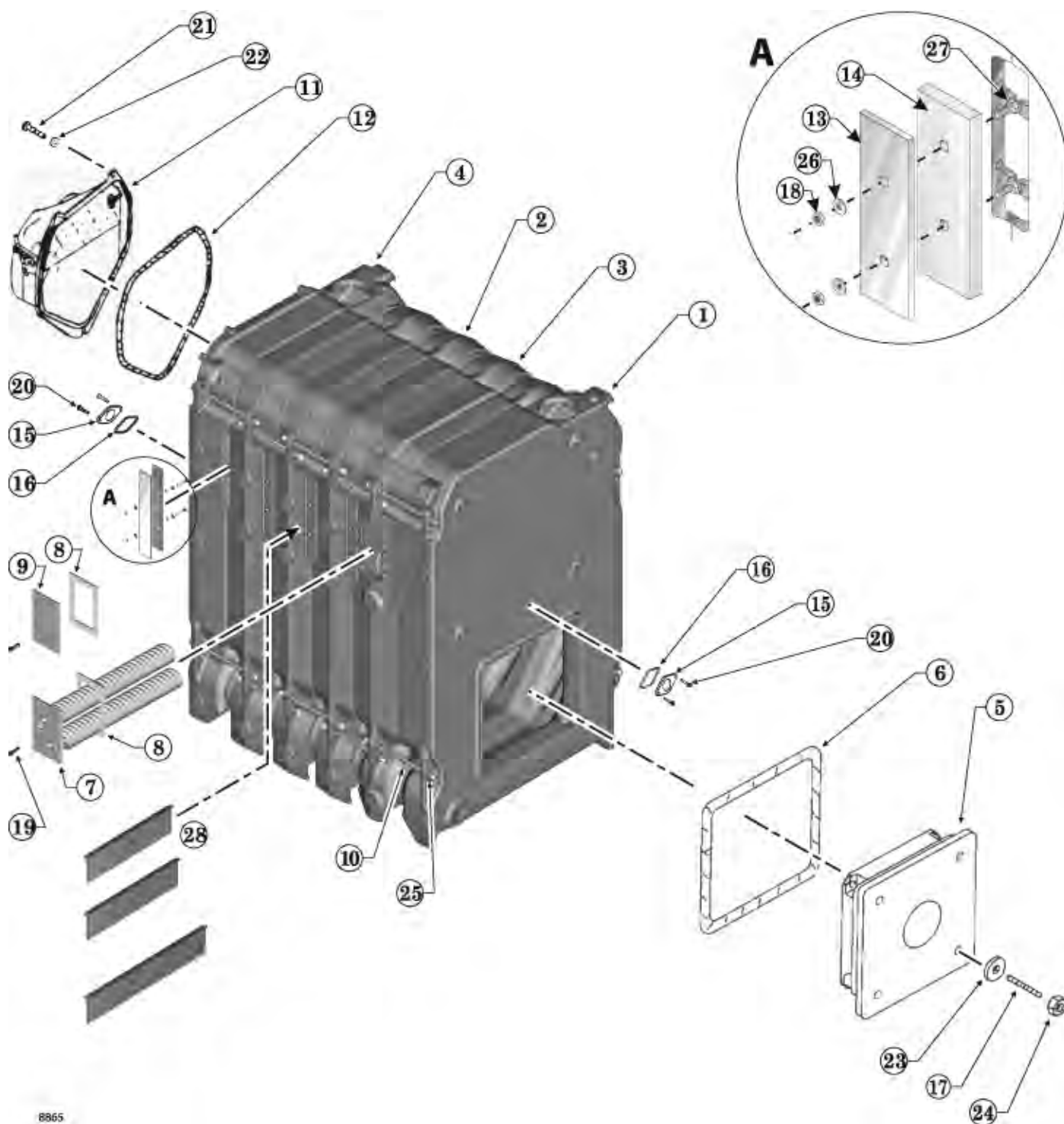
Figure 51 Parts
