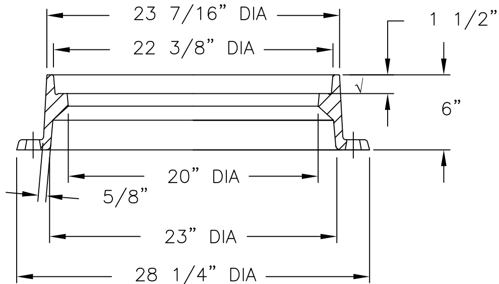
FRAME SECTION
