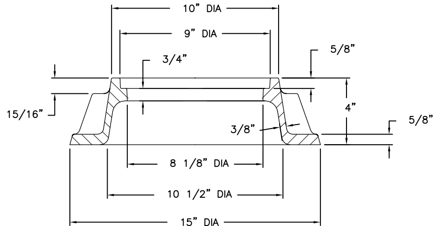
SECTION VIEW
