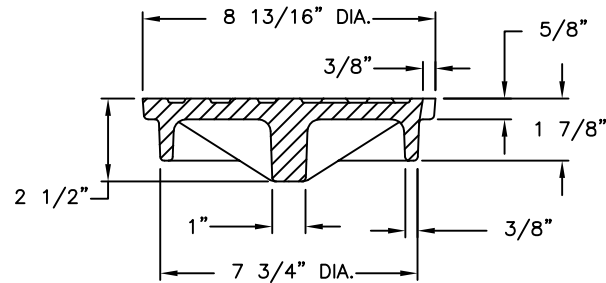
COVER SECTION
