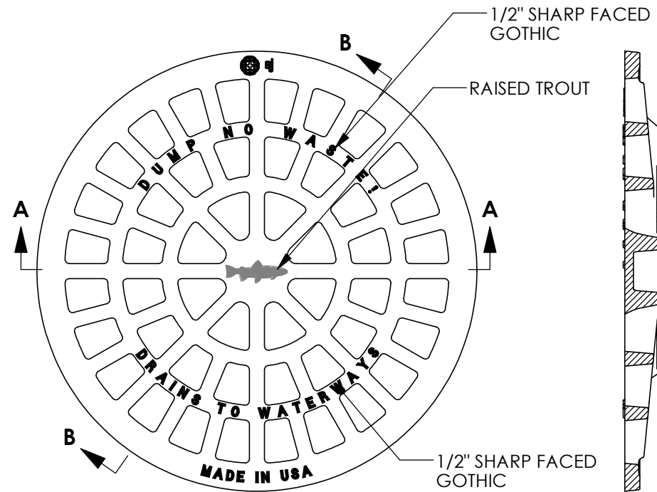
SECTION B-B
