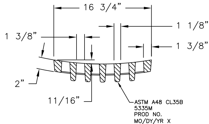
SECTION VIEW
