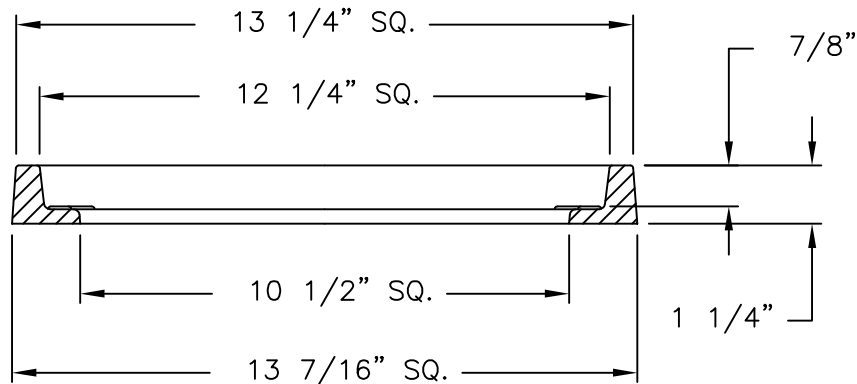
FRAME SECTION
