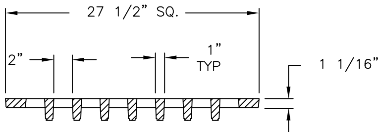
GRATE SECTION
